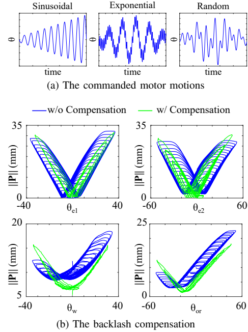
Fig. 7: Example of the commanded motions for validating the backlash compensation and comparison of the backlash compensation for \theta = [\theta_{e1} \ \theta_{e2} \ \theta_w \ \theta_{or}] corresponding to Elbow 1, Elbow 2, Wrist Pitch, and Wrist Yaw with sinusoidal motion.
