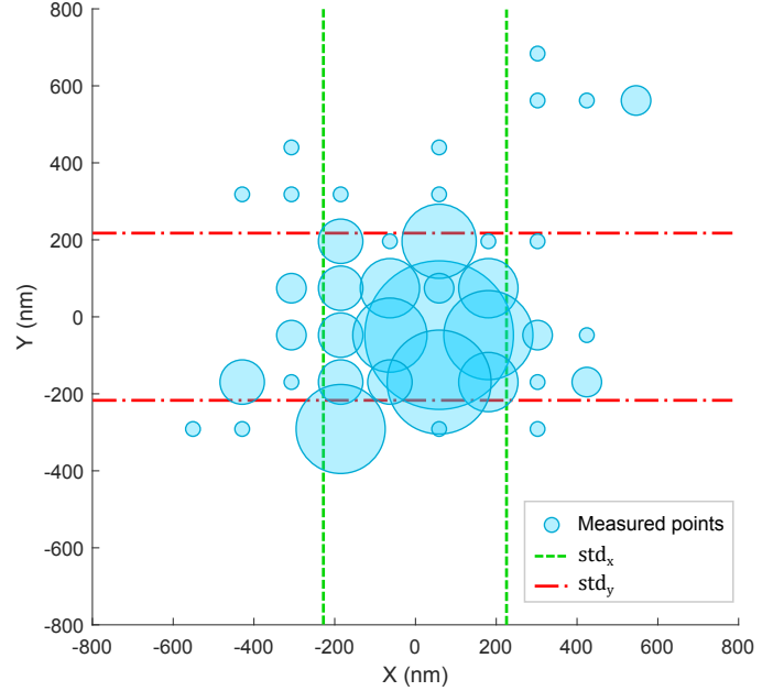
Fig. 8. Repeatability test, distribution of the results of 100 measurements for 20 repetitions of the determined pose (5 measurements per pose), The size of bubble indicates the density of the data measured at that point.
