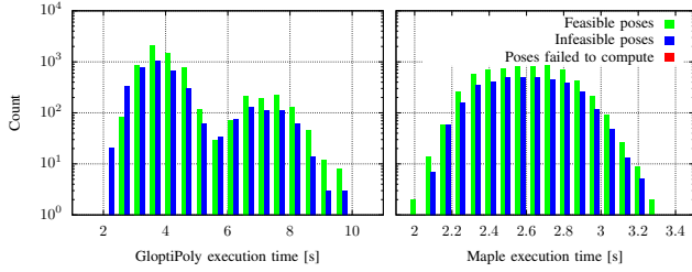
Fig. 2: Histogram of the execution time of (left) the online phase of GloptiPoly, (right) the symbolic reduction and elimination in Maple. Shown results are evaluated on the KUKA LBR IIWA manipulator by the method with the symbolic reduction step (Section VII-A3) for the relaxation order r = 2 and the power of the objective function n = 4 .
