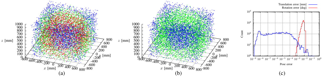
Fig. 1: Generated poses (their positional parts shown only) for the KUKA LBR IIWA manipulator. Green dots are poses marked as feasible, blue as infeasible, and for the red ones, the computation failed. (a) Naïve approach (Section VII-A2). (b) Our method with the symbolic reduction step (Section VII-A3). (c) Histogram of translation and rotation error for the same method as (b). Shown results are for the relaxation order r = 2 and the power of the objective function n = 4 .
