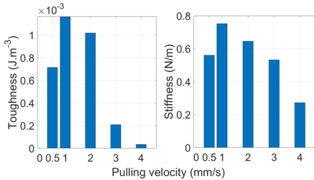
Figure 5: The calculated toughness and stiffness using Fig. 4b for five different experiments with five different fabrication pulling velocities. The toughness and the stiffness are higher when the fabrication pulling velocity is smaller.
