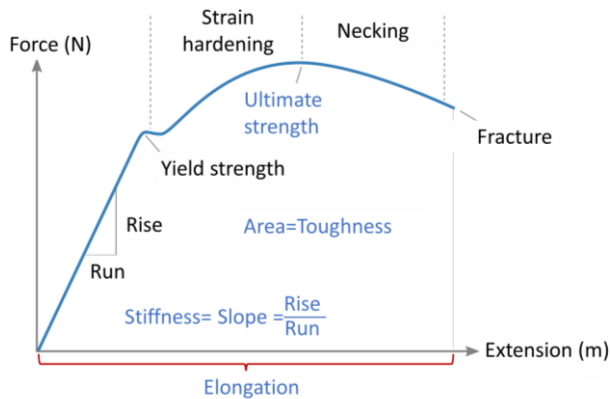
Figure 1: Force-extension curve, obtained by increasingly applying tensile force and measuring the extension. The first linear region is the elastic region, where the force is proportional to the extension and the slope is stiffness. The end of the region is the initiation point of plastic deformation. The force component of this point is defined as yield strength. The second region is the strain hardening. It begins as the force goes behind the yielding point, achieving a maximum at the ultimate strength point, which is the maximal force that can be achieved and is called the ultimate strength. The third region is the necking. A neck develops after the ultimate strength where the local cross-sectional area gets significantly smaller than the average. The necking will increase as the force concentrates more at a small section, which leads to fracture.
