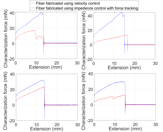
Figure 14: Mechanical properties comparison of the fabricated fibers. The red color represents the obtained characterization force from fiber characterization after fiber fabrication based on velocity control. And the blue color represents the obtained characterization force from fiber characterization after fiber fabrication based on impedance control with force tracking.
