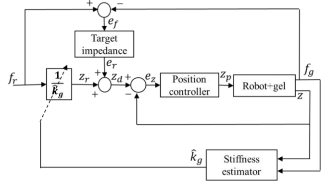
Figure 8: The impedance control with force tracking control scheme applied on fiber threading during the fabrication phase.
