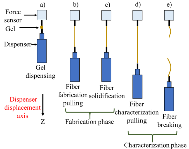
Figure 2: The proposed threading procedure. a) a droplet of gel is dispensed between the tip of the force sensor and the dispenser nozzle; b) the dispenser is moved away from the force sensor pulling the gel droplet into a fiber until certain criteria are satisfied, e.g., displacement or force; c) the system stalls for a certain amount of time to allow the fiber to solidify; d) the fiber is pulled further until e) the fiber breaks.
