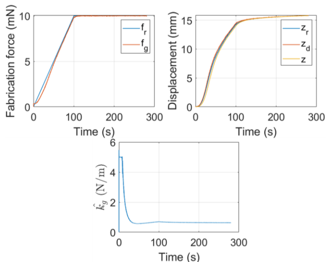
Figure 11: Impedance control with force tracking for fiber fabrication. The fabrication force f_g is compared with the reference force f_r . The fabrication pulling displacement z is compared to the reference z_r and the desired displacement z_d . The corresponding estimation of gel stiffness during threading \hat{k}_g is presented.
