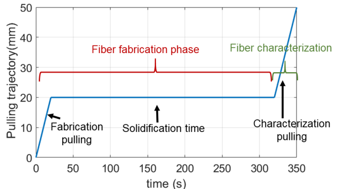
Figure 3: The proposed pulling trajectory for fiber fabrication and characterizations. In the fiber fabrication phase, the gel is pulled continuously and increasing until a given position, where the fiber solidifies for a given solidification time. Then, the fiber characterization phase starts by pulling continuously and increasing until it breaks.
