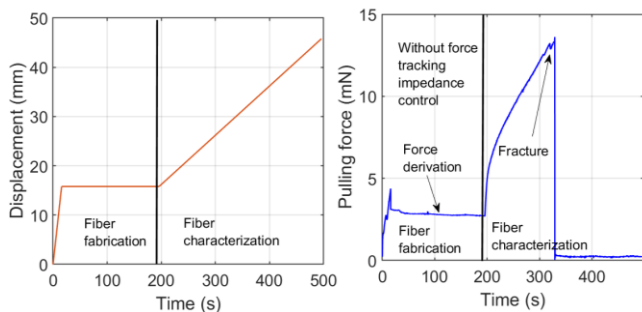
Figure 10: The pulling displacement and applied force profile during the fabrication process, as well as the recorded pulling displacement and force during fiber characterization, based on velocity control.
