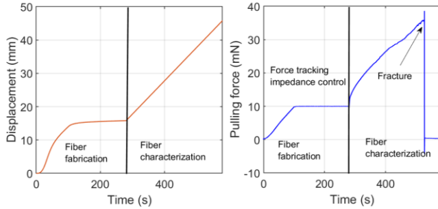
Figure 12: The pulling displacement and the applied force profile during the fabrication process, as well as the recorded pulling displacement and force during fiber characterization, based on impedance control with force tracking.
