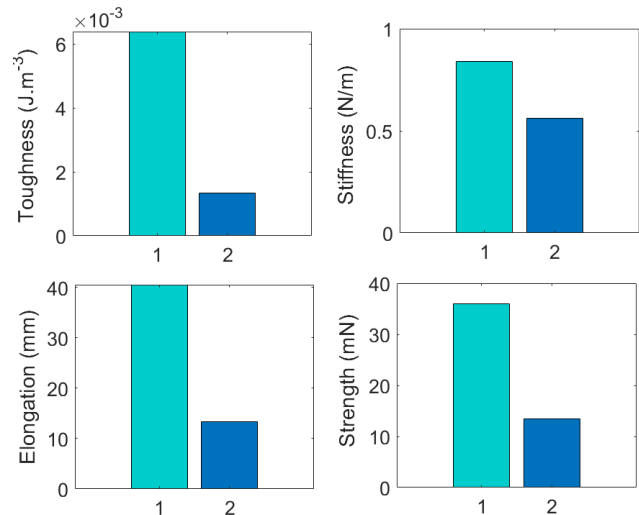
Figure 13: The obtained mechanical properties: toughness, stiffness, elongation, and strength, for fiber fabrication based on impedance control with force tracking (1) and velocity control (2).
