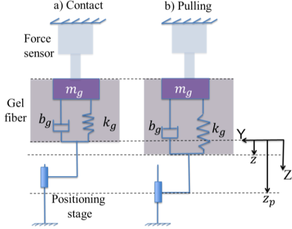
Figure 7: Fiber threading system model based on mass-spring-damper: (a) just at contact f_g = 0 and (b) contact with f_g \neq 0 .
