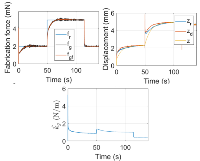
Figure 9: Impedance control with force tracking with an unknown and variable stiffness of the gel during threading. Fabrication force f_g is compared relative to the force reference f_r . The position of the gel z is
