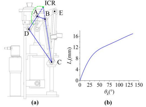
Fig. 2 (a) The four-bar linkage (ABCD) for passive mode. The green dotted line represents the trajectory of the ICR. (b) The length of travel of hydraulic cylinder as a function of knee angle ( L_i(\theta_k) ).
