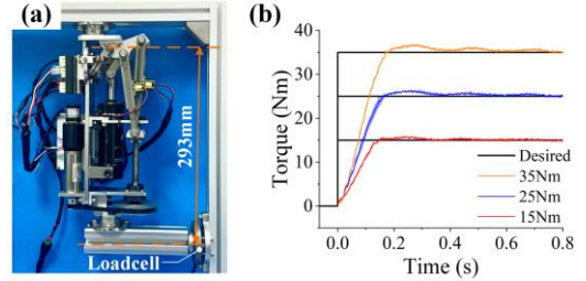
Fig. 10 Bench test for the torque control. (a) Setup for torque step response test. The load cell measuring the reaction force is mounted on the testing jig and the moment arm about joint A is 293mm. (b) The mean and standard deviation of torque step response.
