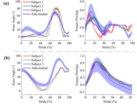
Fig. 13 Results of (a) level-ground walking test in passive mode and (b) stair ascent test in active mode. Trajectories of measured mean knee angle and knee torque of three subjects were compared with the dataset [14] of 22 able-bodied subjects. The shaded areas present the standard deviations. The knee angle in (b) shows small standard deviation because it was obtained in (3) based on encoder data, which was precisely regulated by position control in motor driver.
