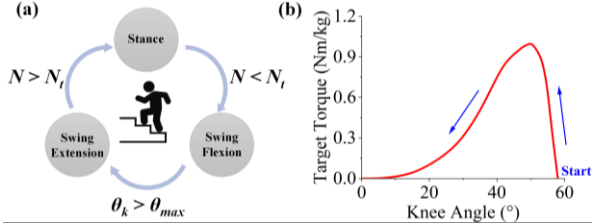
Fig. 8 (a) Phase transition criteria for middle-level control. (b) Torque-angle curve for stance phase control.
