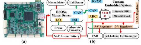
Fig. 7 (a) Top view of the custom embedded system. (b) Block diagram of electrical hardware. The motor driver connects with the embedded system via the CAN bus.
