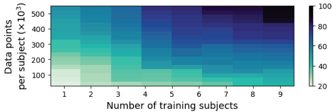
Fig. 9. A heat-map of the classification success rate (%) with regards to the number subjects and the number of recorded data points per subject.
