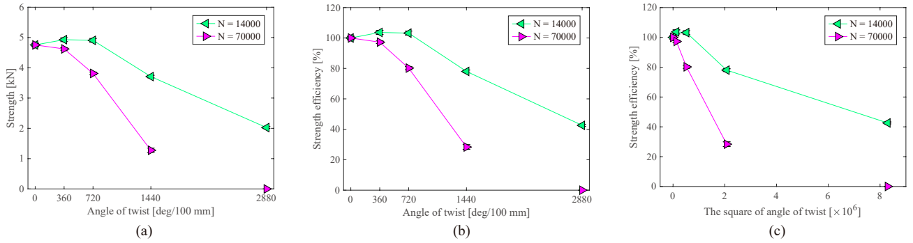
Fig. 5: Relationship between angle of twist and tensile strength or strength efficiency when double \phi 2 mm ropes are placed in parallel. The markers in these graphs show the average value and the error bars show the standard error.
