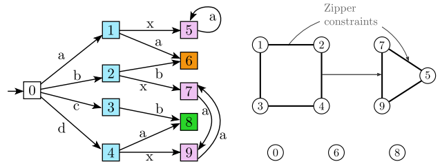
(a) A simple 10-state filter \mathcal{F}_{\text{poly}} , with outputs visualized as colors. (b) Compatibility graph G_{\mathcal{F}_{\text{poly}}} and zipper constraint set.
