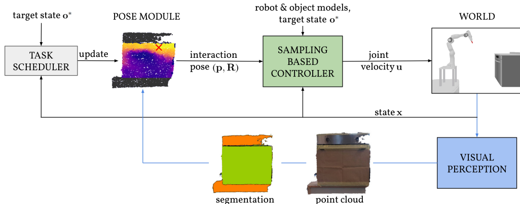
Fig. 2: Block diagram of the control pipeline. The pose module uses affordance estimation to choose the optimal end-effector reference pose. The sampling-based controller generates velocity commands to interact with the object. The task scheduler can trigger an update of the interaction pose if required.
