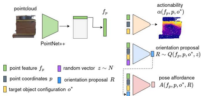
Fig. 3: The pose module, based on [7], combines a PointNet++ [32] feature encoder with three MLP decoding heads, outputting actionability \alpha , orientation proposal Q and pose affordance A .
