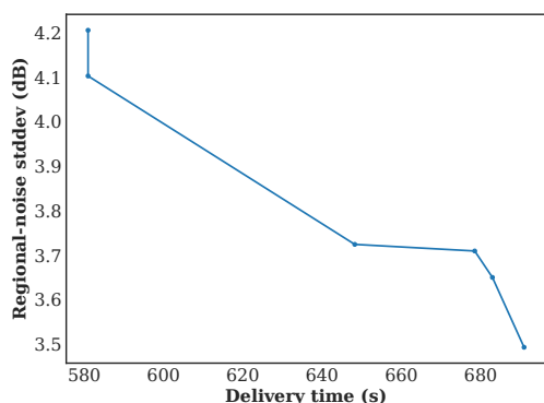
Fig. 7. Trade-off between efficiency and fairness.
