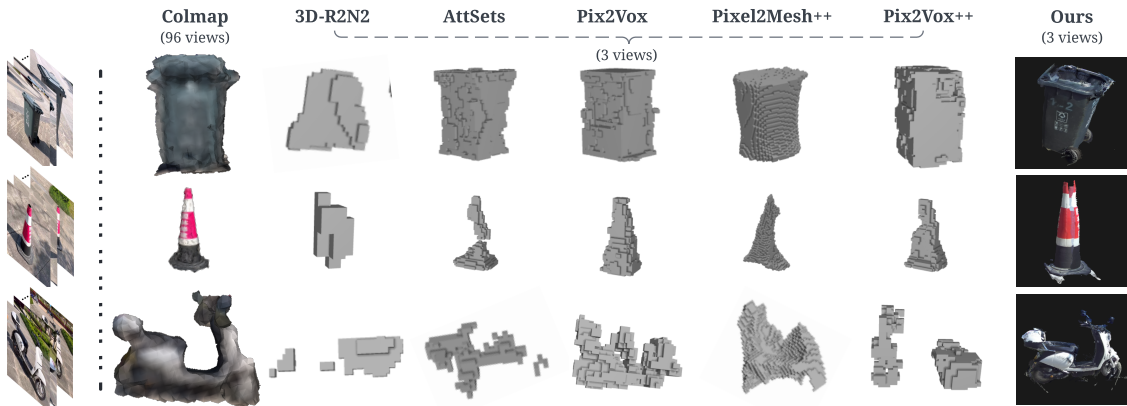
Fig. 4. Comparison of reconstruction effects on outdoor objects
