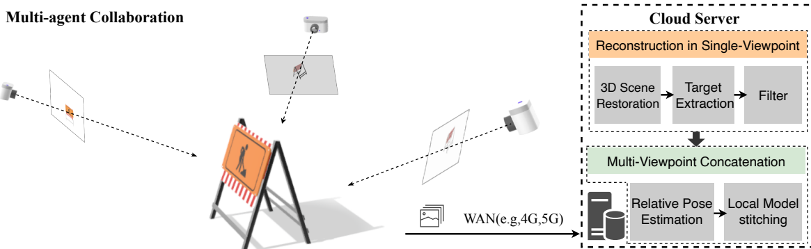
Fig. 1. Several agents detect the target at the same time and upload the observation images from their respective perspectives to the cloud server to complete the object reconstruction. We first recover the 3D scene under each viewpoint and extract the local model belonging to the target object from it. Then, We achieve the concatenation of all local 3D models using the pose estimation parameters generated by aligning the intrinsic features of collaborative agents in the reconstruction space. Note that the figure shows a case where the number of cooperating agents is three.
