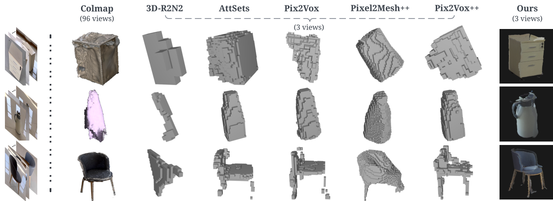
Fig. 3. Comparison of reconstruction effects on indoor objects
