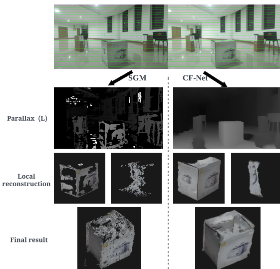
Fig. 5. Comparison of the work of the proposed pipeline under two different parallax acquisition methods.
