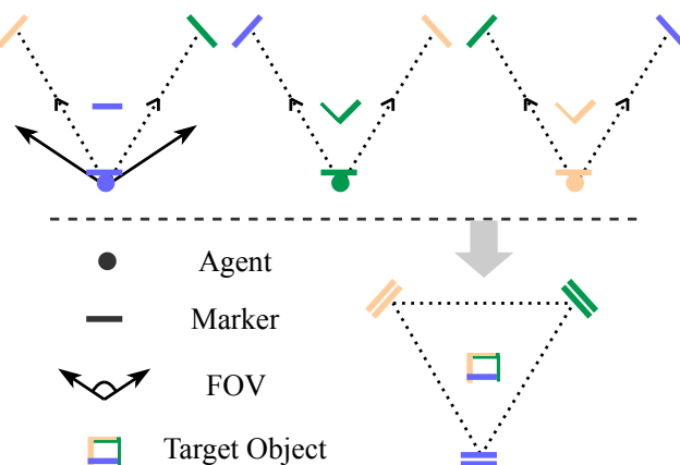
Fig. 2. Bird's-eye view: The local 3D models under various viewpoints can be effectively concatenated through the synchronous alignment of markers.
