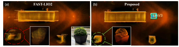
Fig. 6. Point-cloud map of smooth cuboid corridor scene constructed by FAST-LIO2 (a) and the proposed method (b).
