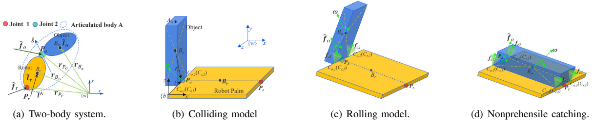
Fig. 2: Hybrid system. B_j is the centroid of body j , and j = r or o denotes robot palm or object. \hat{\mathbf{I}}^A is the spatial inertia of articulated robot-object (simplified as articulated body A ). m_j, \sigma_j are the mass and inertia of body j . \hat{\mathbf{I}}_j \in \mathbb{R}^6 and \hat{\mathbf{f}}_j \in \mathbb{R}^6 are the spatial inertia and the spatial force vector of body j , respectively. \mathbf{r}_{B_j} is the position vector of point B_j . \hat{\mathbf{s}} is joint axis. In the Fig.2(b), (c), (d), C_{r,i} and C_{o,i} , i = 1, 2, 3, 4 are possible contact point pairs. P_j is the equivalent contact point mounted by the virtual joint, and it is also the action point of \hat{\mathbf{f}}_j . \mathbf{r}_o is vector from B_o to P_o . \hat{\mathbf{f}}_{C,i} \in \mathbb{R}^3 are the contact force acted at point C_{o,i} . \{w\} is inertial frame. \{b\} is body frame.
