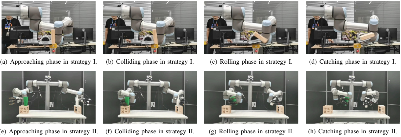
Fig. 6: The experiment setup of strategy I (a-d) and strategy II (e-h) .
