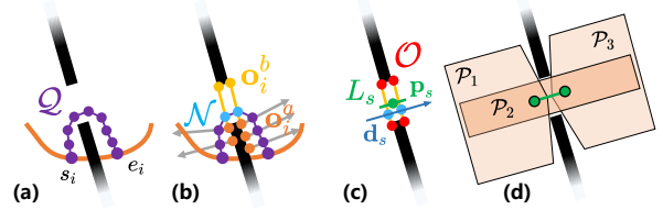
Fig. 5. The proposed line seed generation processes.
