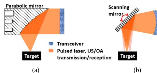
Figure 1. Diagrams showing the different designs of (a) G2 and (b) G3 DMDSM sensors.
