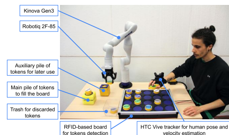
Fig. 4: Setup of filling a tray, the validation task.
