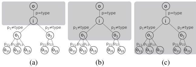
Fig. 3: Graphical representation of the different levels of specificity ( S ) and their respective depth in the knowledge graph. (a) S = 1 , (b) S = 2 , and (c) S = 3 .
