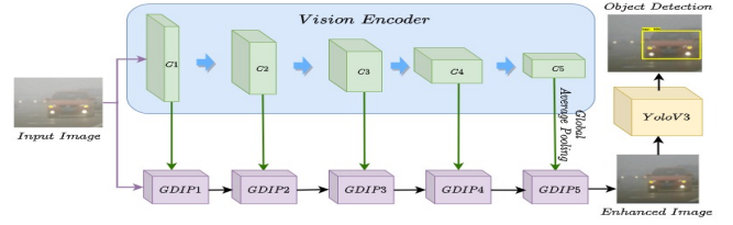
Fig. 3: MGDIP-Yolo : The GDIP blocks perform enhancements progressively on the input image starting with GDIP_1 obtaining intermediate features from C_1 (each GDIP block still performs IP operations concurrently). The final enhanced image is passed to Yolo and the whole pipeline is trained end-to-end.
