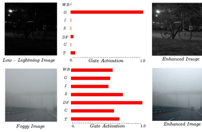
Fig. 6: GDIP gate firing pattern: The bar charts show the gates firing for low lighting and foggy images. GDIP learns the optimum enhancements to apply based on the input image features.
