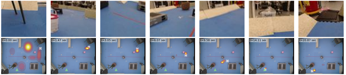
Fig. 5: Localization performance of the agent. Top row: Robot camera images from a successful zero-shot transfer trial. The target is next to the potted plant. Bottom row: Visualization of the robot’s belief over it’s 2D position in the scene, shown as a heatmap on a top-down view of the scene. White X : Ground truth position from motion capture (not input to policy); Green Triangle : Target position.
