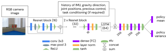
Fig. 4: The policy’s network architecture.
