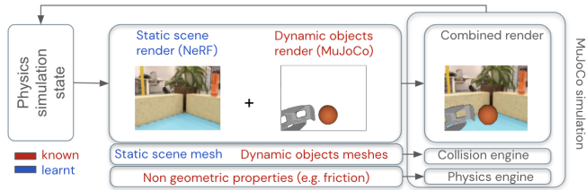
Fig. 3: Our MuJoCo simulation is created by combining: (1) the learnt static scene mesh (Section III-E), (2) the dynamic object meshes and (3) the learnt static scene NeRF rendering (Section III-D) on which (4) the Mujoco rendering of dynamic objects (a ball and robot’s left arm in the camera image above) are overlaid. Other dynamic parameters (e.g. friction) are assumed known or measured.
