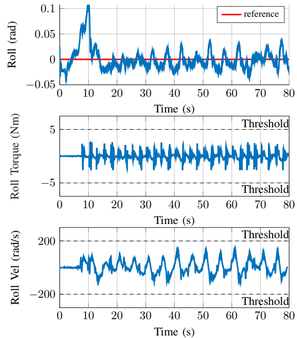
Fig. 6: Roll angle, roll RWA torque, and roll RWA velocity during the hardware beam walking experiment.
