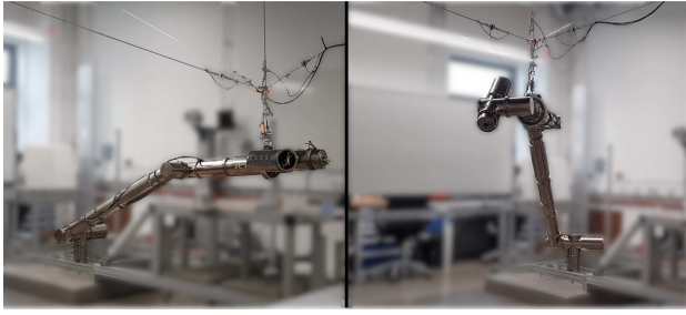
Fig. 8: Motion of CAESAR with the external carrier during the experiment between its initial pose (left) to the final one (right).
