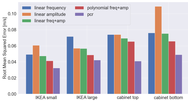
Fig. 6. We tested five different models to estimate drawer speed from sound. Here we analyze their Root Mean Squared Error (RMSE). The PCR model outperforms the other approaches. This indicates that also other features than loudness and pitch of sound are helpful to estimate motion in a drawer.
