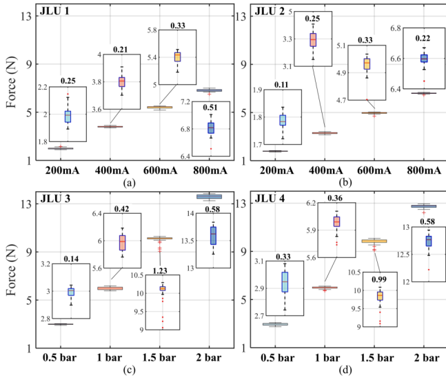
Fig. 7. Results for experiment 3: Box plot for the repetitive precision with regards to forces for (a) JLU 1, (b) JLU 2, (c) JLU 3 and (d) JLU 4. The current of the servo motor for JLU 1 and 2 is set to 200 mA, 400 mA, 600 mA and 800 mA. The current of the motor for JLU 3 and 4 is set to 0.5 bar, 1 bar, 1.5 bar and 2 bar. Each JLU is actuated 30 times. The four insets of each sub-figure are enlarged images for each box plot.
