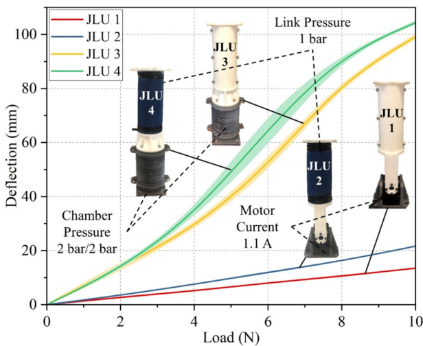
Fig. 4. Results of experiment 1: The red curve and blue curve show the deflection of the JLUs 1 and 2. The actuation current in both motors is 1.1 A. The green and yellow curves show the deflection of the JLU 3 and 4, where the actuation pressure in both VSJs is 2bar. In all cases, the link pressure in the VSLs is 1bar.
