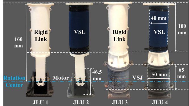
Fig. 1. A set of four joint-link units (JLUs) have been designed, manufactured and compared: a Dynamixel XM430 servo motor (CA, USA) and a rigid link manufactured by SLS 3D printing process with the material of Nylon PA2200 (JLU 1), a motor and a variable stiffness link (VSL) (JLU 2), a variable stiffness joint (VSJ) and rigid link (JLU 3), a VSJ and a VSL (JLU 4). All of these four JLUs have the same rotation centre. The distance between the rotational centres to the tip of the JLUs is 160mm, while the length of the VSL and the rigid link is 100mm.
