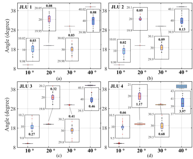
Fig. 6. Results for experiment 3: Box plot for the repetitive precision with regards to the position for (a) JLU 1, (b) JLU 2, (c) JLU 3 and (d) JLU 4. The bending angle of the JLUs are set to 10^\circ , 20^\circ , 30^\circ and 40^\circ . Each JLU is actuated 30 times. The four insets of each sub-figure are enlarged images for each box plot.
