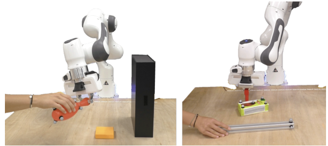
Fig. 1. Experiment settings . Left : Pick-and-place scenario, where the task is to grasp a bowling pin that is arbitrarily handed over to the robot and to place it upright in the middle of the table. Right : Pushing scenario, where the robot has to push the center of the green coffee packet to a moving target location indicated by the tip of the metal stick.
