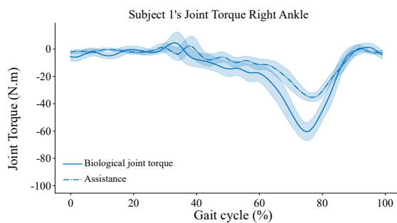
Figure S 3. Joint torque profiles over the gait cycle for the right side of subject 1. The continuous blue line represents the biological joint torque and the dashed blue line is the assistance provided.
