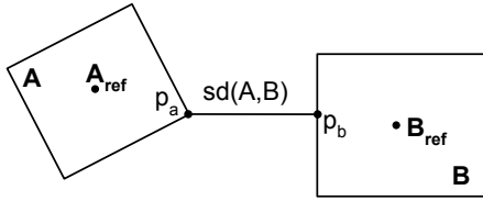
Fig. 4: The reference points on the convex hulls used to get the distance function output.
