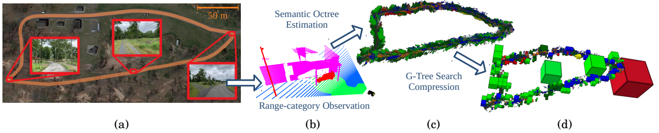
Fig. 2: Summary of the semantic octree building and compression framework. (a) The robot navigates in a large, semantically-rich, outdoor environment. (b) Range-category observations are gathered to build a semantic octree of the environment (c) that is then compressed by G-tree search (d). While shown here sequentially, the semantic octree estimation and G-tree search compression may run concurrently as described in Section III. Colors in the trees (c)-(d) correspond with semantic classes.
