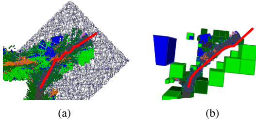
Fig. 5: (a) The optimal path found by COA* in the graph constructed with a Halton sequence. (b) The optimal path found by COA* in the graph constructed based on the compressed octomap nodes.
