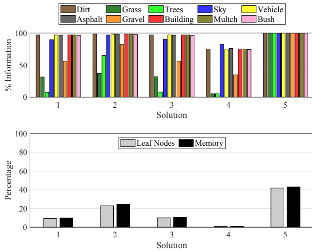
Fig. 3: (top) Percentage of information retained for each semantic class as a function of the G-tree search weights (solution number) with respect to the corresponding quantities in the finest-resolution tree \mathcal{T}_W . (bottom) Percentage of leaf nodes and approximate memory required to store the compressed tree relative to the corresponding values of the finest resolution octree \mathcal{T}_W . Memory results assume each tree node requires 256 bits of memory.
