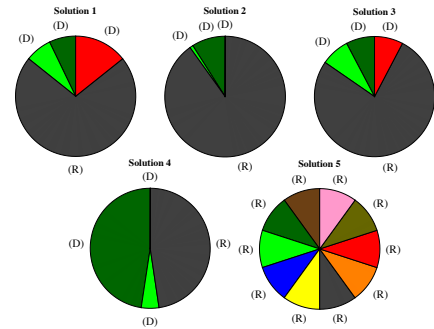
Fig. 4: Weights for G-tree search. Colors correspond with the semantic class coloring, (R) is a relevant class, and (D) is an irrelevant one. In solutions 2 and 4, the (D) near the top corresponds to the red class (building). Note that classes marked (R) have weights \beta_i , whereas those marked (D) have weights \gamma_j in (1). Classes not shown have weight zero.
