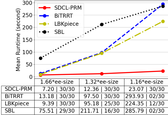
Fig. 5: Compare 7-DOF scenes with different hardness levels. Table is showing “average runtime (s) | solved cases”. 30 trials for each planner and each difficulty level.
