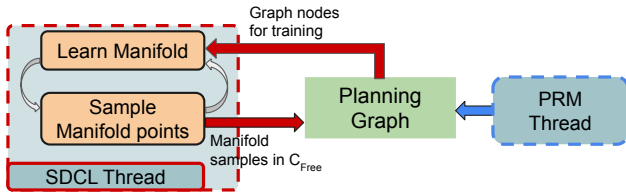
Fig. 2: Block diagram of SDCL. The planning graph is shared between two threads. Both threads contribute to the graph, and the SDCL thread uses the graph for training. todo: change graph to SDCL
