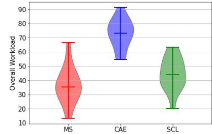
Fig. 8: NASA Workload Index.
