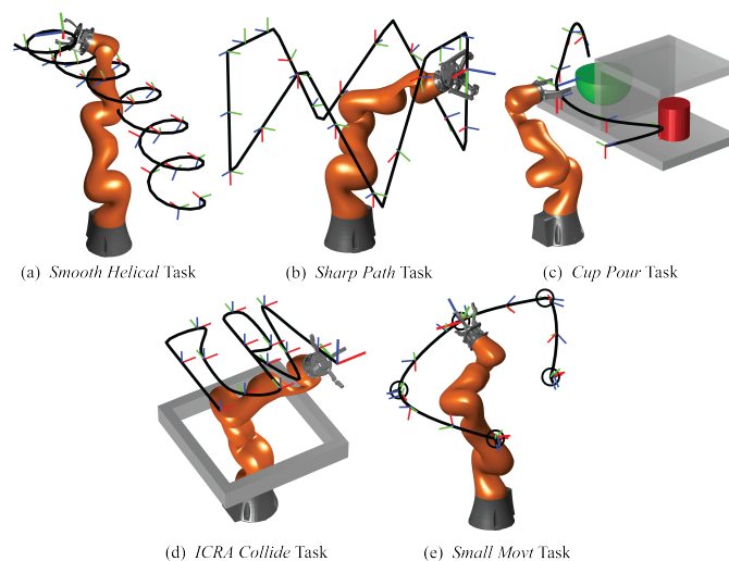
Fig. 2. Experiment tasks used to evaluate the arm-hand combinations on the various configuration quality objectives, such as ability to avoid collisions, maintain pose accuracy, smooth out motion, and so on.
