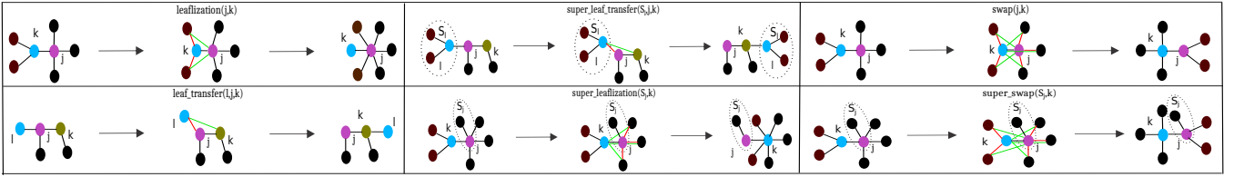
Fig. 2: (a) L(j, k) , (b) LT(l, j, k) , (c) SLT(S_l, j, k) , (d) SL(S_j, k) , (e) swap(j, k) , and (f) super\_swap(S_j, k) operations.
