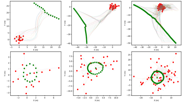
Fig. 1: Trajectory visualizations for line and star formations for 15, 30, and 60 robots, column-wise. Initial positions and final positions are represented by red and green colors, respectively.
