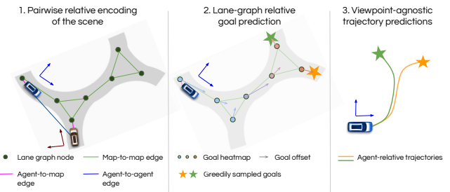
Fig. 1. Our model, GORELA, encodes the scene by reasoning about pair-wise relative geometric relationships between the agents and the lane graph with a GNN. Then, it predicts a goal distribution using the lane graph nodes as anchors, and samples goals from it. Finally, trajectories are generated conditioned on the goals. The architecture is viewpoint-invariant, thus allowing for shared computation across agents.
