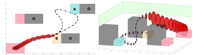
Fig. 3: Drone delivery, top down (left) and side (right) views.
