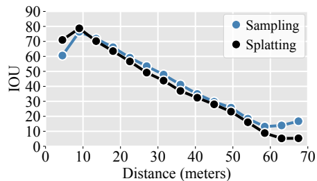
Fig. 2: Comparing IOU over distance for Lift-Splat-style splatting versus our bilinear sampling strategy: splatting is better at close range, bilinear sampling is better at long range.
