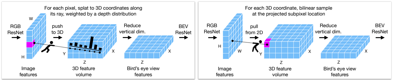
Fig. 1: 2D-to-BEV architecture, illustrated with two lifting strategies. The left panel shows the Lift-Splat approach [10]: in this method, each 2D feature is “pushed” to 3D, filling voxels that intersect with its ray. The right panel shows our bilinear sampling approach: in this method, each 3D voxel “pulls” a feature from the 2D map, by projection and subpixel sampling.
