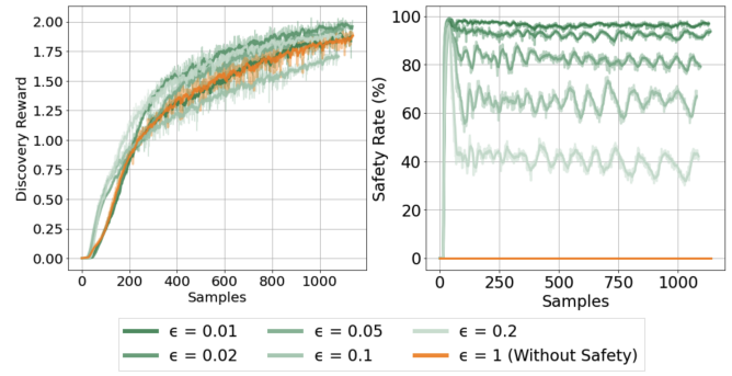
Fig. 3: Reward and safety rate during skill discovery phase.
