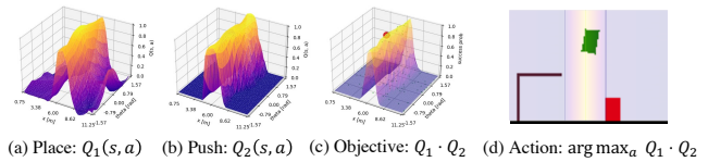
Fig. 2: Planning in a 2D toy domain. The agent needs to get the green block under the brown receptacle with two skills: Place() and Push() that operate on the horizontal position x of the green block. Plots (a) and (b) show the Q-functions across (x, \theta) for each skill. Place() is only trained to get the green block on the ground, so the planner must determine a = x s.t. Push() is unobstructed. The optimal action maximizes the probability of long-horizon task success (Eq. 2), approximated by the product of Q-functions in plot (c).
