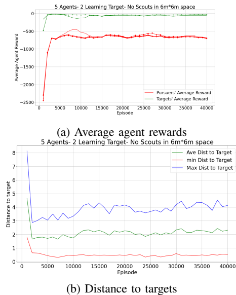
Fig. 2. Rewarding and distance-to-target metric for Multi-Target MADDPG (with 5 pursuers vs. 2 evaders)
