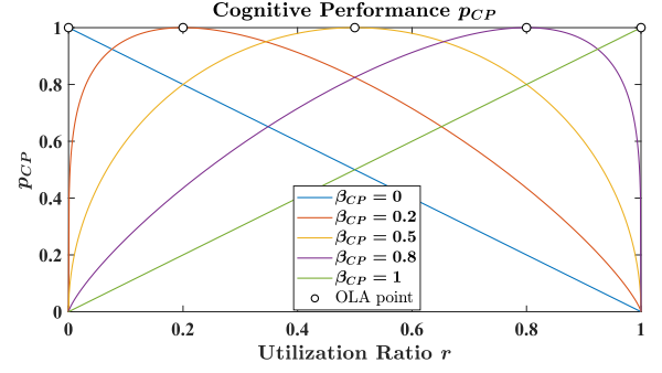
Fig. 3. Examples of the Cognitive Performance p_{CP} versus utilization ratio r with different levels of task difficulty \beta_{CP} (13).
