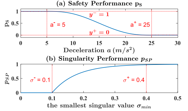
Fig. 2. (a) An example of the Safety Performance p_S versus deceleration a (4) when x^- = a^- = 5 , x^+ = a^+ = 25 , y^- = 1 and y^+ = 0 . (b) An example of the Singularity Performance p_{SP} versus the smallest singular value \sigma_{min} (6) when \sigma^+ = 0.4 , \sigma^- = 0.1 and \varphi = 0.02 .
