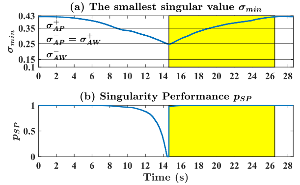
Fig. 6. (a) The smallest singular value \sigma_{min} . (b) The Singularity Performance p_{SP} . Yellow shaded area is the prediction on whether the robot is heading away a singular configuration based on (7).
