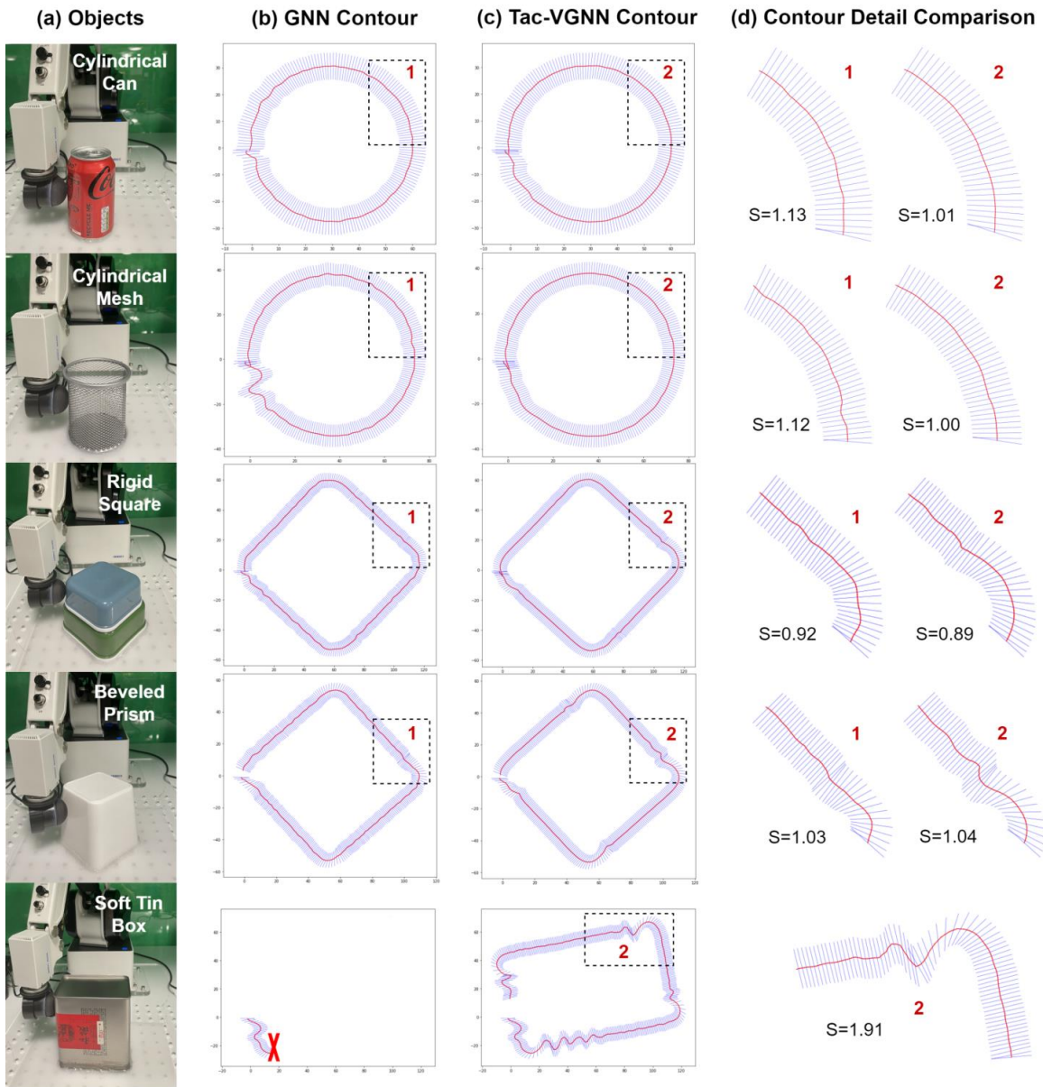
Fig. 10: Comparison of surface servoing with different objects: (a) real scene when tactile servoing starts; (b) the trajectories for the GNN model, which fails when servoing around the soft tin box; (c) the trajectories for the Tac-VGNN model which is the best overall; (d) zoomed-in comparison of trajectories and local smoothness values.
