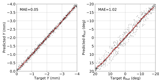
Fig. 9: Tac-VGNN model test performance for surface pose estimation, including perpendicular depth Y and rotation angle \theta_{Roll} .
