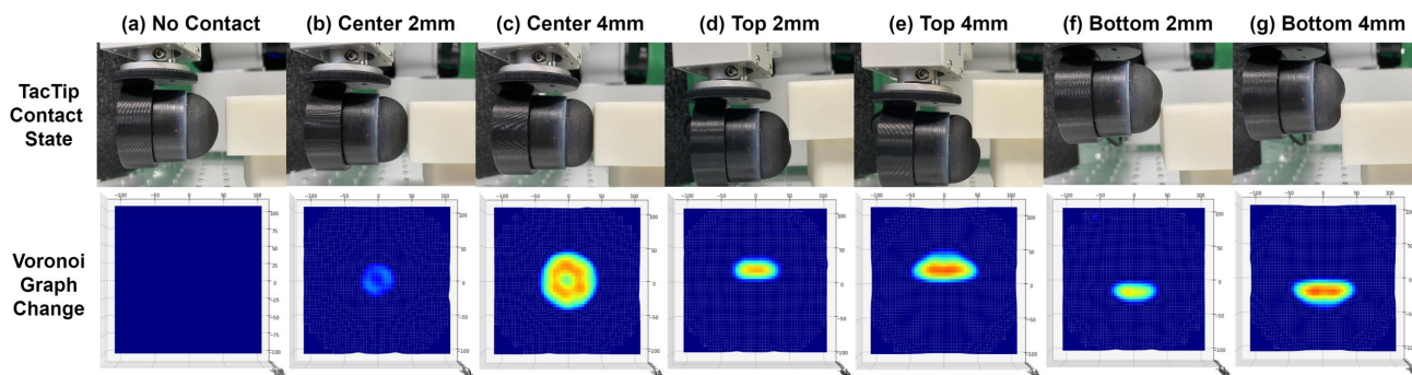
Fig. 8: Data interpretability comparison: (a) the reference state without contact, \{Y = 0mm, \theta_{Roll} = 0deg\} ; (b,c) the TacTip central area contacts the surface at different depths, \{Y = [2, 4]mm, \theta_{Roll} = 0deg\} ; (d,e) and (f,g) the TacTip peripheral area touches the object at the top and bottom respectively, \{Y = [2, 4]mm, \theta_{Roll} = 0deg\} .
