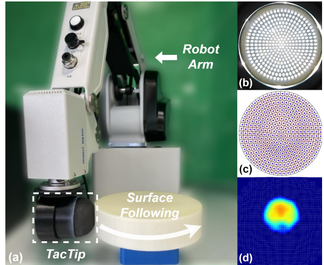
Fig. 1: Overview of the experimental setup and the Voronoi Graph for tactile servoing. (a) shows the surface following task conducted by a low-cost desktop robot arm (Dobot MG400) and a tactile sensor (TacTip). (b) displays the raw image comes from the TacTip sensor. The concept of ‘tessellation’ can be illustrated in (c). The change of Voronoi enhanced graph data (d) have strong explainability on X, Y, and Z dimension.
