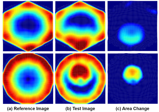
Fig. 4: 3D plots of Voronoi graph after interpolation operation: (a) shows the reference data which has no contact; (b) represents the Voronoi graph data when deformation occurs; (c) displays the difference between the images in the first and second column.
