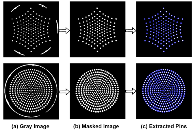
Fig. 2: Tactile data preprocessing: (a) the cropped grayscale tactile image; (b) application of circular mask of suitable size to remove artifacts from lighting; (c) pin positions extracted by blob detection.
