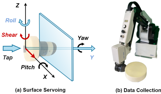
Fig. 6: Illustration of pose definition and data collection process. (a) required pose parameter for surface servoing task; (b) an example of data collection using a robot arm. In terms of pose \{Y, \theta_{Roll}\} , the collection setups have a range of \{[-2, 2]mm, [-30, 30]deg\} . The tap range is 5mm along Y . Shear is added in \{X, \theta_{Roll}\} with range \{[-5, 5]mm, [-5, 5]deg\} , facilitating model robustness and generalizability. The number of collected data is 5000.
