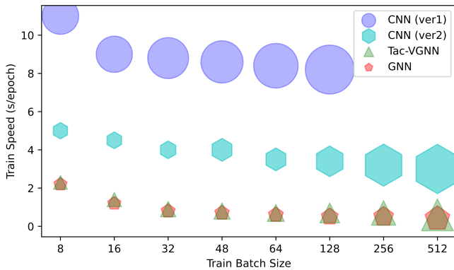
Fig. 7: Comparison of model training efficiency. The training time per epoch based on different batch sizes of four models is shown on the diagram. The size of four kinds of markers indicates the GPU memory usage during training for different models.
