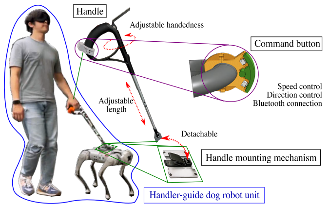
Fig. 4. Harness handle interface design that features speed and direction control button, adjustable handle, and detachable structure for portability.
