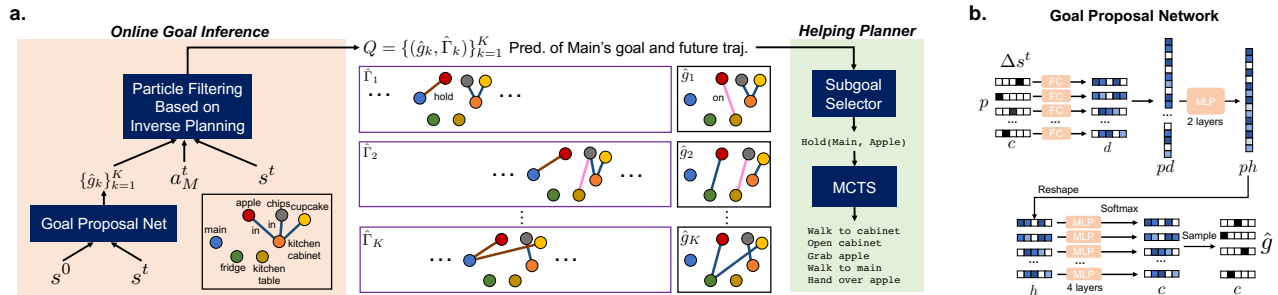
Fig. 2: (a) Overview of our approach, which consists of an online goal inference module and a helping planner. We represent states and goals using scene graphs. s^t is the state at time t ; a_M^t is the main agent’s action at time t ; \hat{g}_k is the k -th goal proposal; and \hat{\Gamma}_k is the prediction of the main agent’s future trajectory corresponding to \hat{g}_k . (b) Goal proposal network. \Delta s^t is a matrix encoding the difference between the predicate counts in the states s^t and s^0 , where each row is a one-hot vector, indicating the change in the count of a specific predicate. p = 136 is the number of all predicate types, c = 9 is the maximum number of counts, and d = 100 and h = 128 are the dimensions of the intermediate layers.
