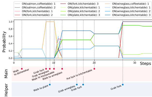
Fig. 5: Goal inference and plans by NOPA for the same task shown in Fig. 4c, which is setting up a kitchen table for 3 persons. We show the posterior probabilities of the top predicates and their counts based on the particles at each step, key actions of the main agent (indicated by red dots), and key helping actions (indicated by blue dots). At step 2, after watching the main agent walking towards the dishwasher, NOPA rejects proposals involving nearby objects (e.g., apples, salmons) that are not inside of the dishwasher. After the main agent grabs a fork at step 8, NOPA infers with high confidence that the goal is setting up a table for at least one person. So at the following step, the helper agent takes its very first action – walking to grab a plate. Upon seeing Main walking to the kitchen table at step 10, the goal location becomes certain. After observing more actions, the inference converges to setting up the kitchen table for 3 persons.
