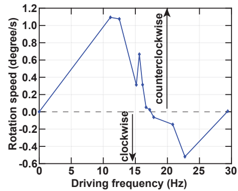
Fig. 13. Frequency dependence of rotation speed.
