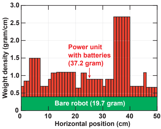
Fig. 7. Non-uniform weight distribution of the robot, including a bare robot (actuators, substrate, and foam feet) (green) and the electronics on flexible PCB, including the microcontroller and batteries (red).
