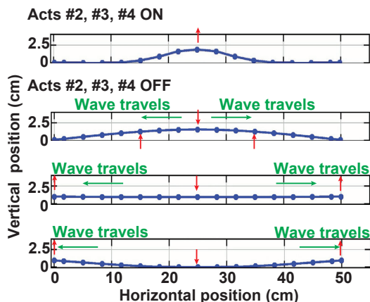
Fig. 6. Traveling waves propagating along the robot. Snapshots of the robot's shape over time are simulated and plotted. Voltages of actuators #2, #3, and #4 are turned on and off. Traveling waves transmit from the midsection to the ends, which ultimately lift up as a result.
