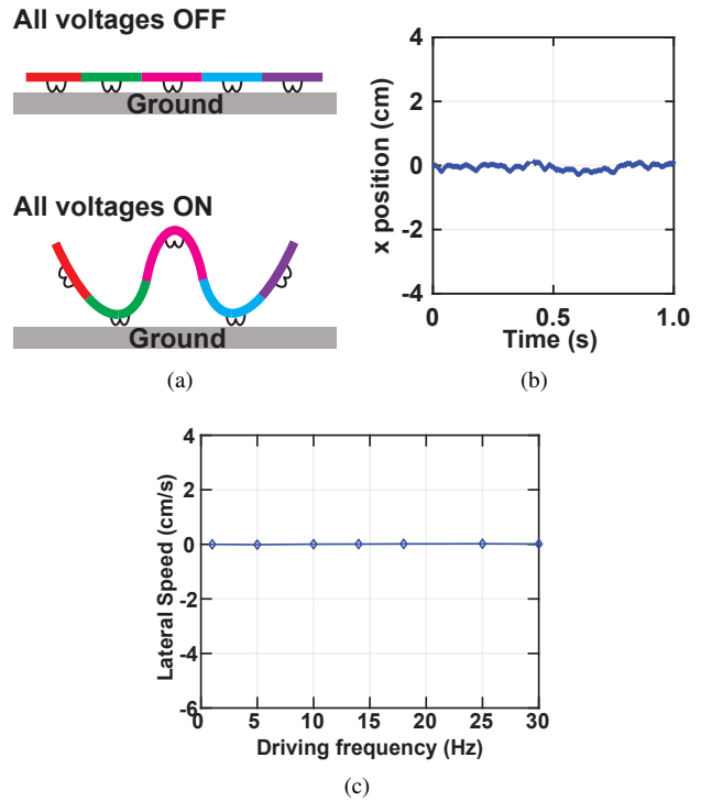
Fig. 9. (a) Robot setup and (b) the horizontal movement over time for a uniformly-loaded setup (bare robot, only comprising the actuators and feet). (c) Frequency dependence of the robot's lateral speed, with the uniform setup in Fig. 9a.
