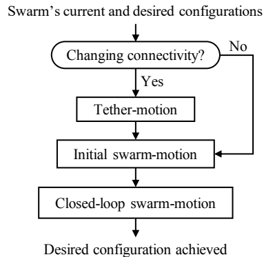
Fig. 3. Proposed tether-based swarm-motion control strategy.
