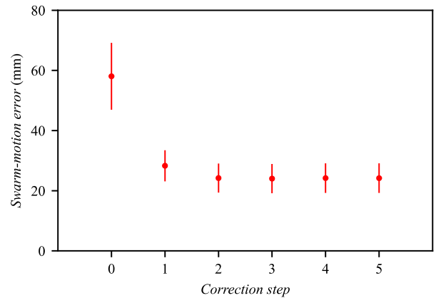
Fig. 8. Closed-loop motion control for one desired swarm configuration.
