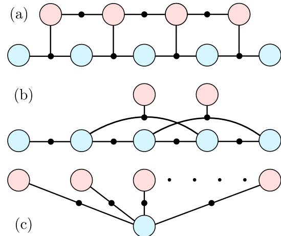
Fig. 1. Discrete-continuous factor graphs in robotics. Factor graphs modeling several relevant discrete-continuous robot perception problems. Discrete variable nodes are colored red, continuous variable nodes are blue, and factor nodes are black. (a) Switching systems: discrete states control the evolution of a continuous process. (b) Outlier rejection: discrete inlier/outlier variables control whether a subset of untrusted measurements should be used in estimating continuous variables. (c) Point-cloud registration: discrete variables represent correspondences and the continuous variable is the relative transformation from a source to target point-cloud.
