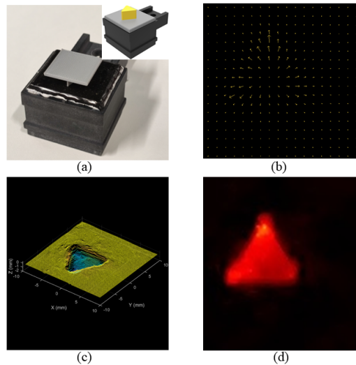
Fig. 1. (a) A triangular test indenter makes contact with the DelTact [7] tactile sensor. (b) The captured tactile flow (plotted sparsely for visualization). (c) The reconstructed 3D contact point cloud. (d) The depth map extracted from (c).
