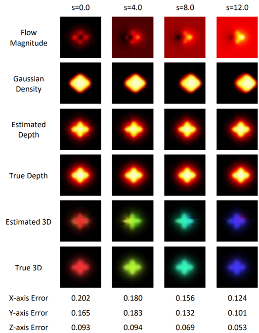
Fig. 4. The result with FEM simulated data. The estimated and true depths refer to the z axis displacement of the point cloud. For the flow magnitude, the Gaussian density, and depth, brighter color means a larger numerical value. For the 3D point cloud, the displacements in XYZ axes are regarded as the HSV color channels, respectively.
