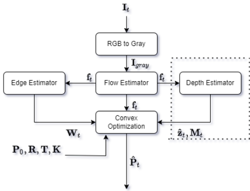
Fig. 2. The pipeline for solving the 3D point cloud reconstruction problem. Arrows denote signals and blocks denote processing modules. The dotted region is possible to be replaced with some other method or sensing modality to provide depth information to constrain the optimization.
