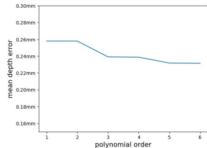
Fig. 5. The depth regression error from the Gaussian density using polynomial order up to 6.
