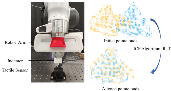
Fig. 7. The experimental setup of the pose estimation experiment.
