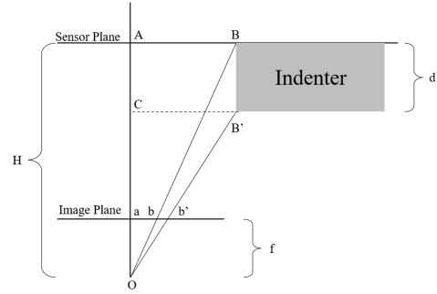
Fig. 3. A simplified projection graph for the sensor surface deformation resulted from a rectangle indenter. After the indentation, point B on the original sensor surface moves to point B'. This results in point b in the image going to point b'. The indentation depth is d, and the camera's focal length is f. The distance from the sensor plane to the optical center is denoted as H.
