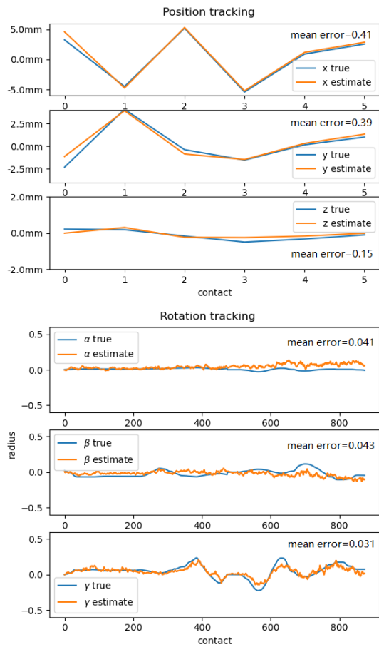
Fig. 8. The robot arm returned (regarded as ground truth) positional change and orientation change (represented in Euler angles) with the ICP estimates. For positional tracking, discrete contacts are made. For rotational tracking, contact is made solid and continuous. The mean tracking errors are shown on each plot.
