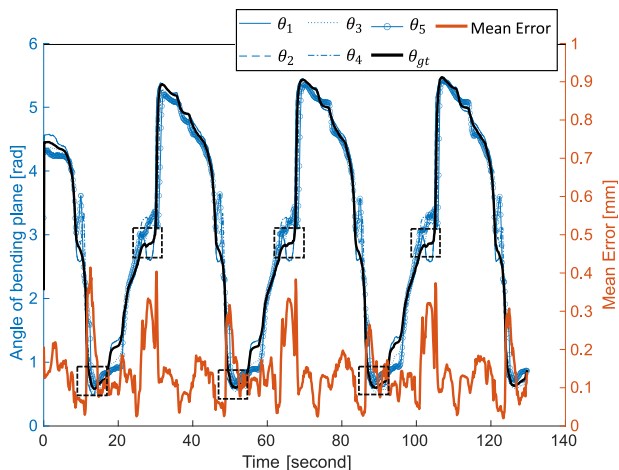
Fig. 13. The estimated angles of the bending plane of each grating (blue), ground truth angle of the bending plane (black) and mean error (orange) of lissajous (1) experiment are plotted over the time. The transition regions where there are increases in mean error are marked with dashed square.
