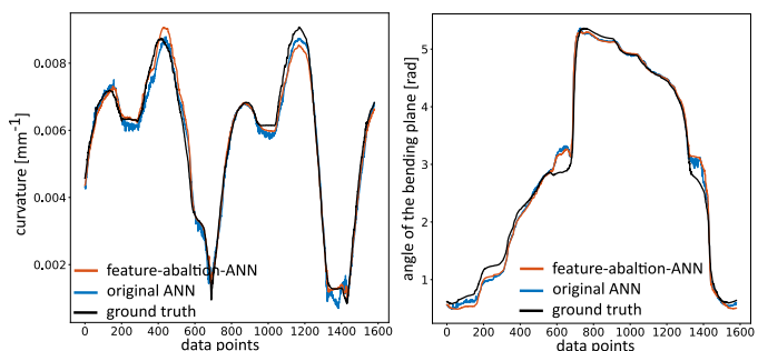
Fig. 10. The results of the feature ablation study. The feature-ablation-ANN (with three inputs) and the original ANN (with four inputs) trained for grating set 3 were evaluated on testing trajectories lissajous (1). The feature-ablation-ANN could achieve a comparable performance as the original ANN even if the information from the central core is not provided.
