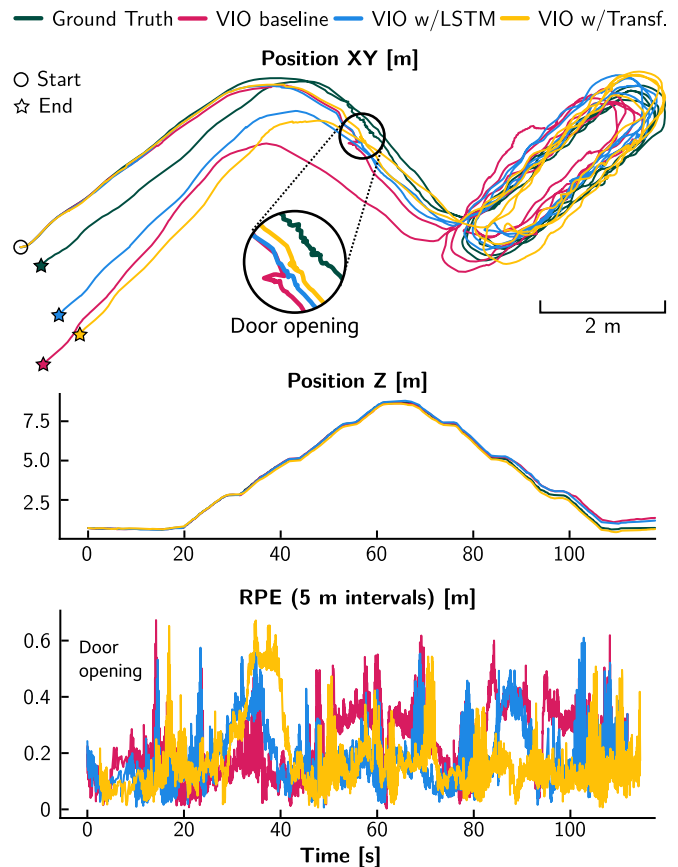
Fig. 8. NCD-Multi Stairs results. Top : Position of the baseline VIO, LSTM and Transformer methods on xy -plane. We magnify the door opening section of the trajectory where the baseline clearly diverges due to loss of visual feature tracking and poor bias estimation. Middle : Position of the trajectory for the z -axis. Bottom : 5 m RPE for each algorithm.
