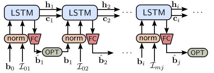
Fig. 5. LSTM architecture. A IMU data window \mathcal{I}_{m,j} of size w (with m = j - w ) and the previous bias \mathbf{b}_i are first normalized then passed to the LSTM. The hidden state is preserved for the next inference step and the output is passed through a fully connected layer to predict a bias.
