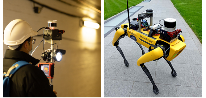
Fig. 1. Two of the platforms used in this work. Left: handheld device including a SevenSense AlphaSense visual-inertial sensor. Right: the same device mounted on a Boston Dynamics Spot quadruped. An IMU bias model from a neural network trained on handheld data was used to infer the biases on the Spot dataset without any retraining — despite the significantly different motion pattern. The lidar was not used in these experiments.
