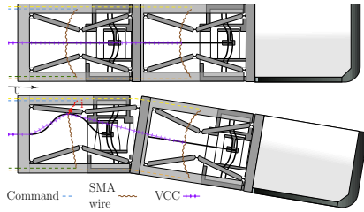
Fig. 11. Schematic representing routing and operating principle.
