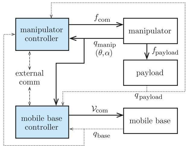
Fig. 6. Overview of each Omnid's control system. The solid lines indicate communication channels used in this paper. The dashed lines indicate optional wireless communication with a centralized controller or other Omnids. The dotted lines indicate optional exteroceptive sensing of the payload and mobile base configurations.
