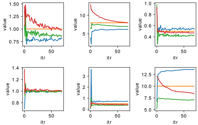
Fig. 4: We randomize the order of agents during the inverse learning problem and the cost parameters converge consistently regardless of the order of iterations and the initial conditions. Each plot corresponds to one learned parameter and different colors represent a different initial condition or the order of iteration. X axis is the number of iterations and Y axis is the parameter value.
