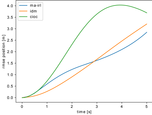
Fig. 6: Root Mean Square Error for the predicted trajectories using the INTERACTION data set.
