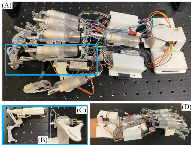
Fig. 1. (A) overview of the exoskeleton glove system, (B) index finger linear Series Elastic Actuators (SEA), (C) rotary SEA, (D) user wearing the exoskeleton glove. Blue – enlarged view of index finger linear SEA and rotary SEA.
