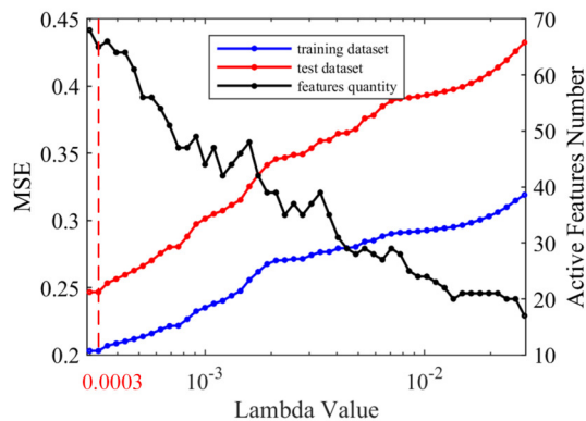
Fig. 18. The comparison of MSE on training dataset and test dataset, and active features number with different \lambda_d value.
