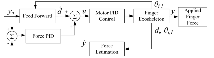
Fig. 9. Force control scheme for a single exoskeleton finger. \theta_{i,1} represents the MCP joints of exoskeleton finger i ( i \in \{1, 2, 3, 4, 5\} ). d_i represents the current motor position of exoskeleton finger i .
