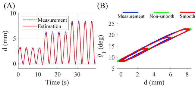
Fig. 14. (A) The comparison between the estimation of motor current position and measurement from encoder. (B) The comparison between the estimation of motor current position and measurement from encoder, related to MCP joint angle \theta_1 .
