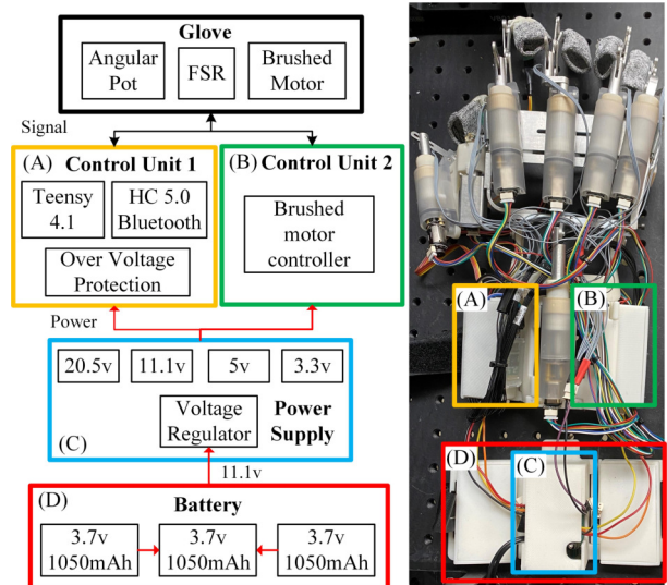
Fig. 7. Electronics design overview: (A) micro-controller board, (B) brushed motor controller board, (C) power conversion board, (D) 3-in-1 battery package.
