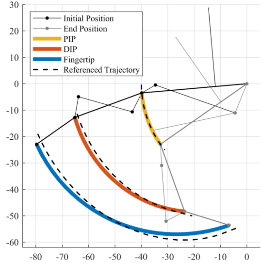
Fig. 4. Kinematic simulation of the optimized index finger exoskeleton rotating around the MCP joint from 5^\circ to 35^\circ . The trajectories of the PIP joint, DIP joint, and fingertip are shown. The referenced trajectories, which are based on the referenced joint angle with a selected finger length, are also shown for comparison.
