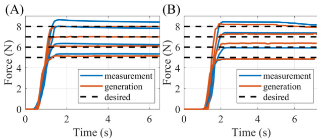
Fig. 23. The comparison between desired force, measured force and generated force. (A) shows the experimental results on horizontal platform ( \theta_1 = 14.9^\circ ) and (B) shows the experimental results on vertical platform ( \theta_1 = 21^\circ ).
