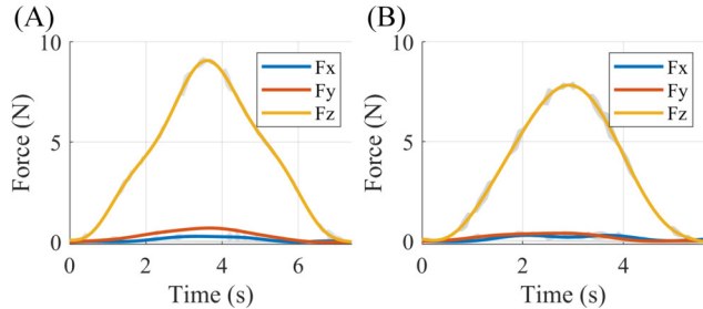
Fig. 13. (A) Force measurement with load cell horizontal installation ( \theta_1 = 12^\circ ). (B) Force measurement with load cell vertical installation ( \theta_1 = 25^\circ ).
