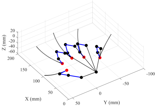
Fig. 5. Simulation of a small diameter cylindrical grasp with optimized finger linkages. The blue bars represent the exoskeleton links. The black dots represent the exoskeleton joints. The red dots represent the endpoints of each linkage. The dotted lines represent the trajectories of the fingers' motion.
