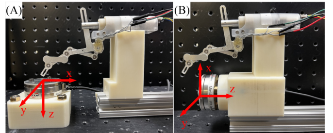
Fig. 11. Test platform with different load cell mounting positions. (A) load cell is mounted horizontally. (B) load cell is mounted vertically.
