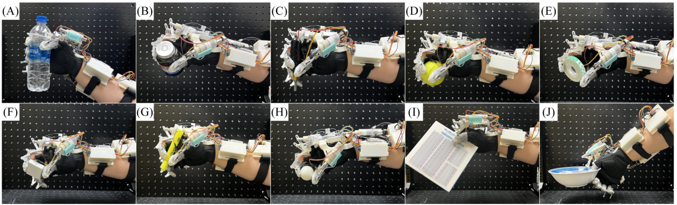
Fig. 24. Examples of successful grasps of each object. Each object is grasped 5 times by a single participant. (A) bottle, (B) jar, (C) screw driver, (D) ball, (E) tape, (F) small box, (G) pen, (H) small ball, (I) flat box, (J) bowl.
