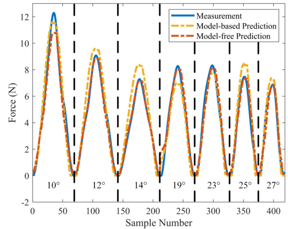
Fig. 16. Force prediction results on test dataset with different \theta_1 configurations. Each configuration is performed once. Different configurations are not time related.
