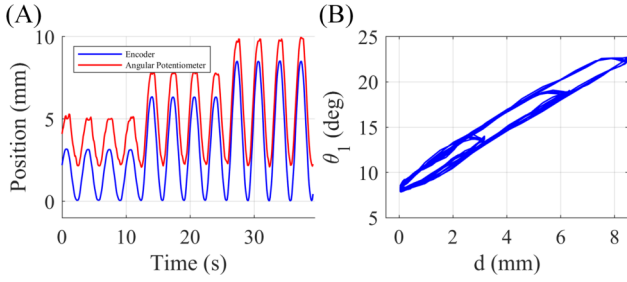
Fig. 8. Backlash illustration. (A) The motor position calculated by encoder and angular potentiometer separately, (B) The relationship between the motor position d and the MCP joint angle \theta_1 .
