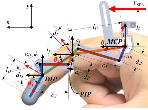
Fig. 2. Mechanism schematic and kinematic model of the index exoskeleton finger linkage. Different colors represent different links: Blue link – Distal phalanx, Green link – Intermediate phalanx, Orange link – Proximal phalanx, Brown links – constraint links.
