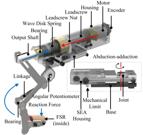
Fig. 3. Perspective View of the index linkage. The screw nut guided by leadscrew connects to the output shaft. The compressed wave disk spring between the output shaft and screw nut measures the force by its deformation when the fingertip makes contact with an object. The red arrow shows the force generation flow and the blue arrow shows the force measurement flow. The distal link is adjustable and can be extended by 7mm. The LSEA can slide on the base to accommodate different hand size. The partial view shows the details of the abduction-adduction mechanism. It is implemented at the bottom of the SEA to connect the finger linkage with the base through a joint. At the initial position, the hand needs to be open and be ready for grasping. The spring on the side pulls the exoskeleton finger linkage to the side to perform the abduction. Mechanical limits were added to avoid excess force to the fingers. The palmar interossei muscle group will perform the adduction automatically and stretch the spring while grasping.
