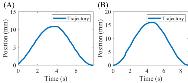
Fig. 12. (A) The LSEA motor position trajectory with load cell horizontal installation ( \theta_1 = 12^\circ ). (B) The LSEA motor position trajectory with load cell vertical installation ( \theta_1 = 25^\circ ).
