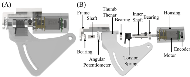
Fig. 6. Design of RSEA for thumb thenar: (A) Perspective view of the RSEA, (B) Exploded view of the RSEA.
