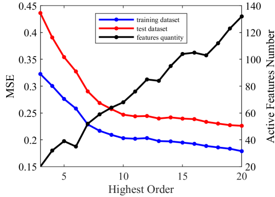
Fig. 17. The comparison of MSE on training dataset and test dataset, and active features number with different highest polynomial order.
